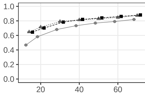
Reliability of ICCs
