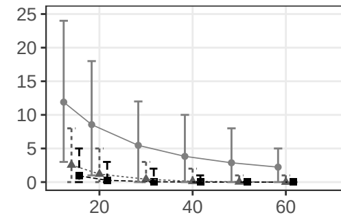
Number of Negative ICCs
