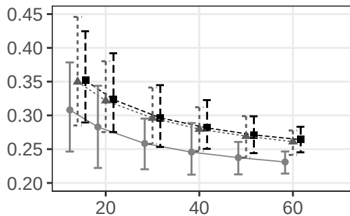
SD of ICCs
